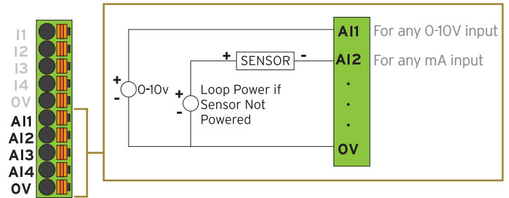
INPUT CONNECTOR
