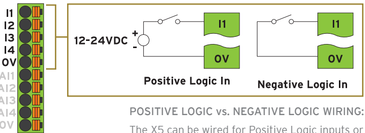
INPUT CONNECTOR
