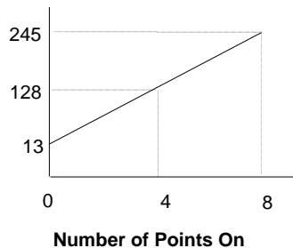
Maximum Current Drawn from Backplane (mA)
