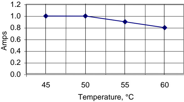
3.3V Output vs. Ambient Temperature
