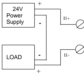
Current Source
