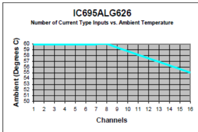
Figure 1: Thermal Derating
